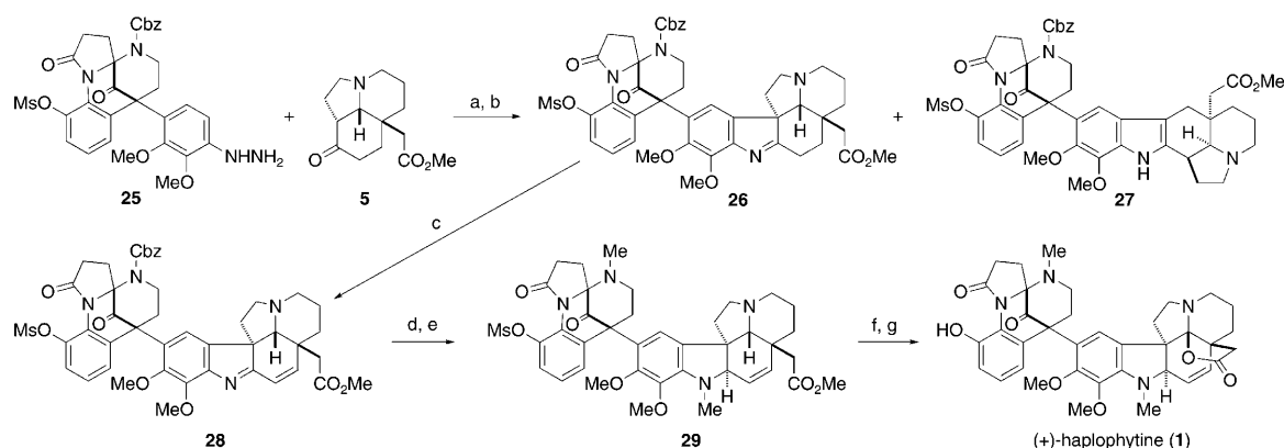
Scheme 5. Completion of the total synthesis of (+)-haplophytine ( 1 ). Reagents and conditions: a) 50 % aq H 2 SO 4 , 1,4-dioxane, 0 °C, 80 %; b) p TsOH, t BuOH, 80 °C, 47 % of 26 and 29 % of 27 ; c) benzeneseleninic anhydride, THF, reflux, 61 %; d) BBr 3 , pentamethylbenzene, CH 2 Cl 2 , –78 °C to –25 °C, 67 %; e) HCHO (37 %), NaBH 3 CN, AcOH, CH 2 Cl 2 /MeOH (1:1), –78 °C to RT, 55 %; f) 1 M NaOH, MeOH, 60 °C; g) K 3 [Fe(CN) 6 ], NaHCO 3 , t BuOH/H 2 O (1:2), 0 °C to RT, 70 % (2 steps).
